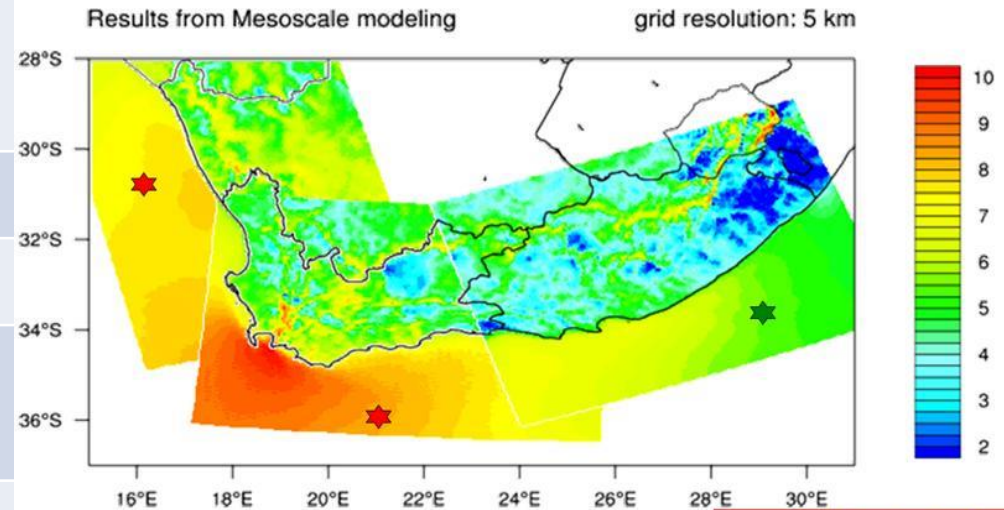
Mean wind speed (m/s) at 50 m – KAMM/WASP, 3 domains
